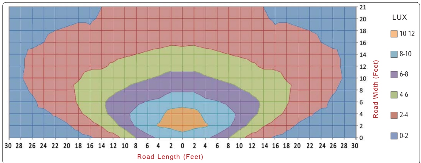
LUX Distribution Pattern
